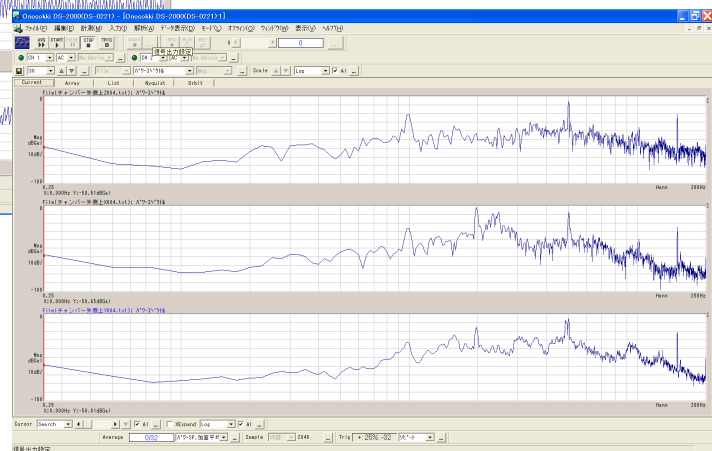
Acceleration spectrum ( frequency: 0-200Hz axis: X,Y,Z)
