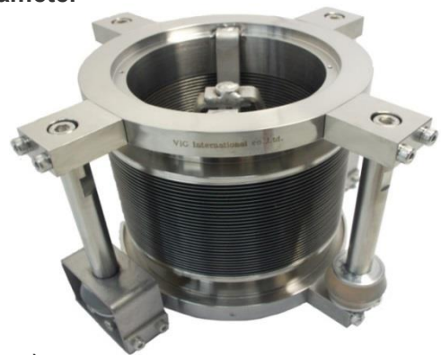
ISO100 Vibration Free Damper Model: VTD-100ISO
