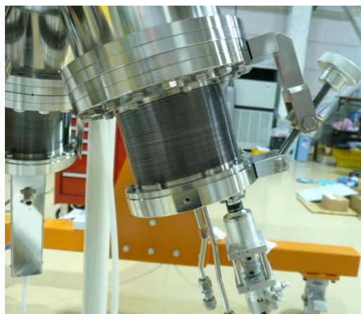
3-inch splutter gun with inclined bellows
