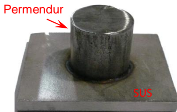
Permendur-SUS Good result of liquid penetrant test
